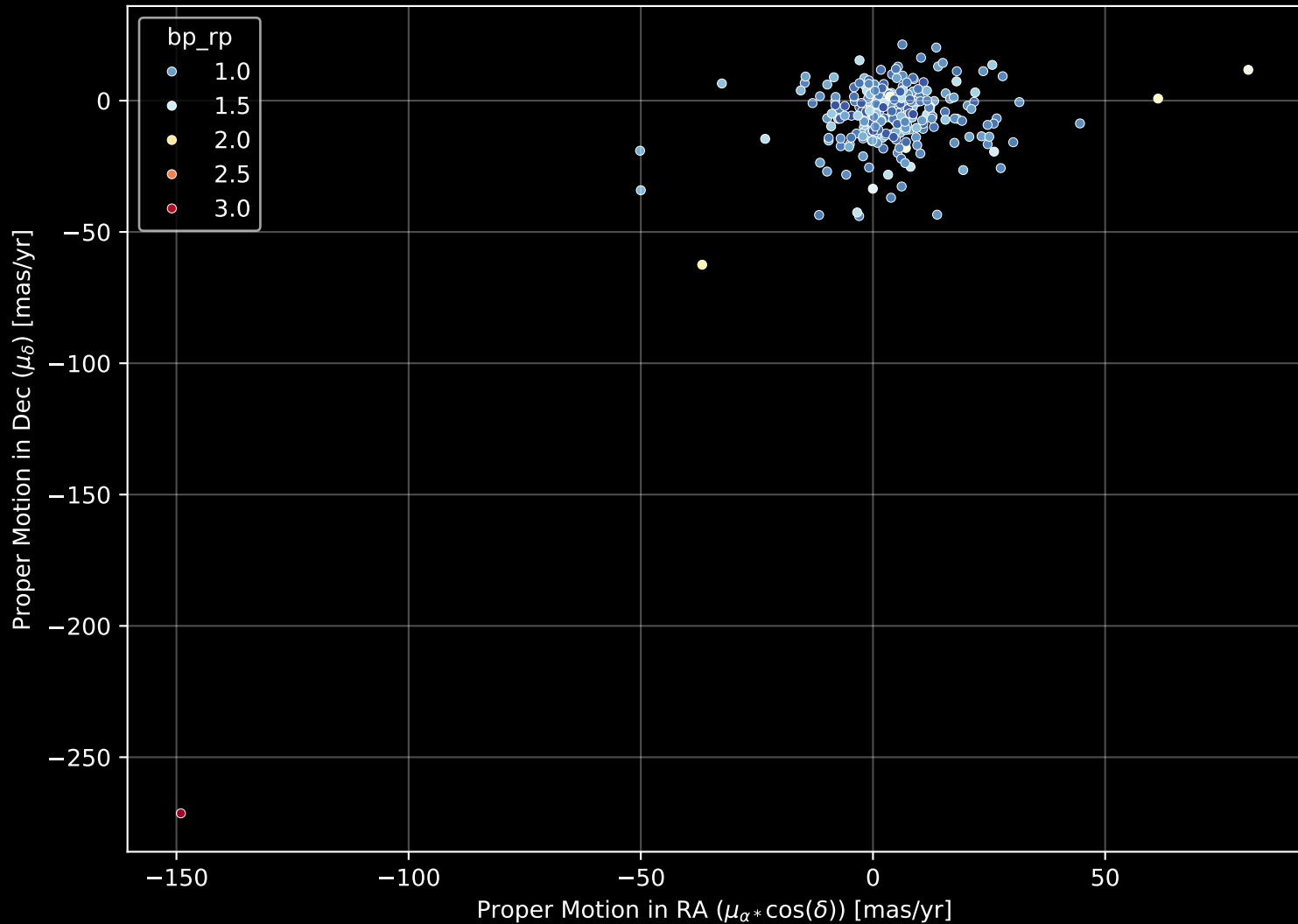
GALAH DR4 Field: [750] Proper Motion Diagram (n= 268)
