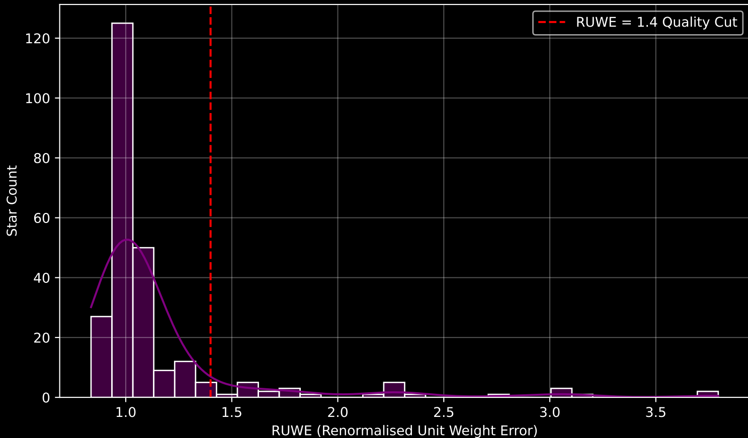
GALAH DR4 Field [750] RUWE Distribution (n= 254)
